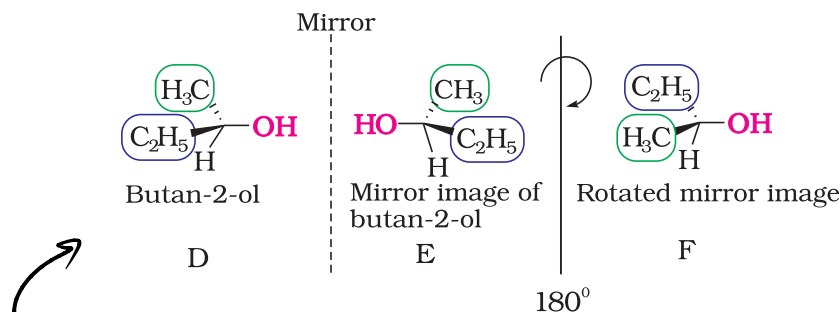
Fig 6.6: E is mirror image of D; E is rotated by 180° to get F and F is non superimposable on its mirror image D.
